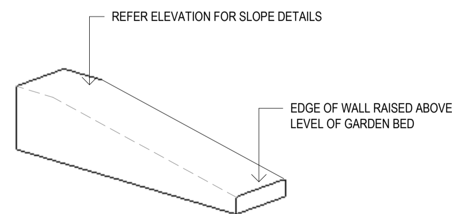
3 LWA-001 TYP2 - INSITU CONCRETE SEATING WALL Copy 1
