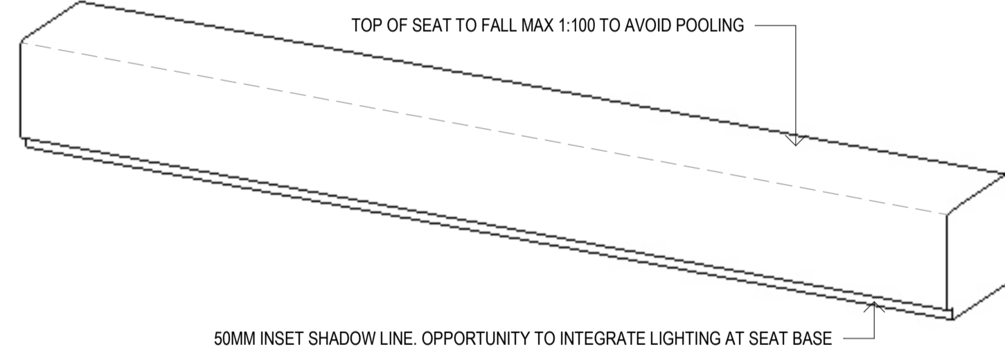
2 LWA-001_TYP1 - INSITU CONCRETE SEATING WALL Copy 1
