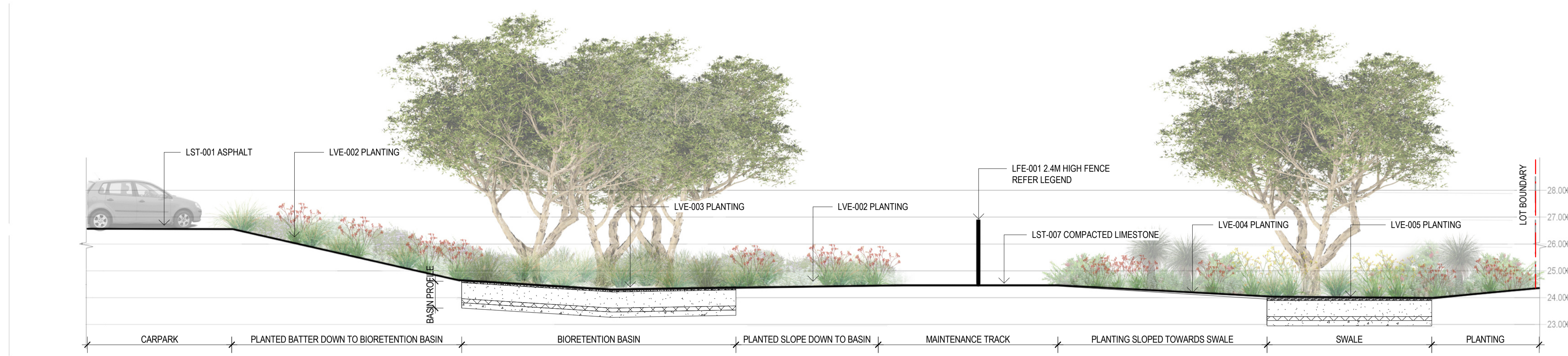
1 EASTERN EDGE INTERFACE 1:100
