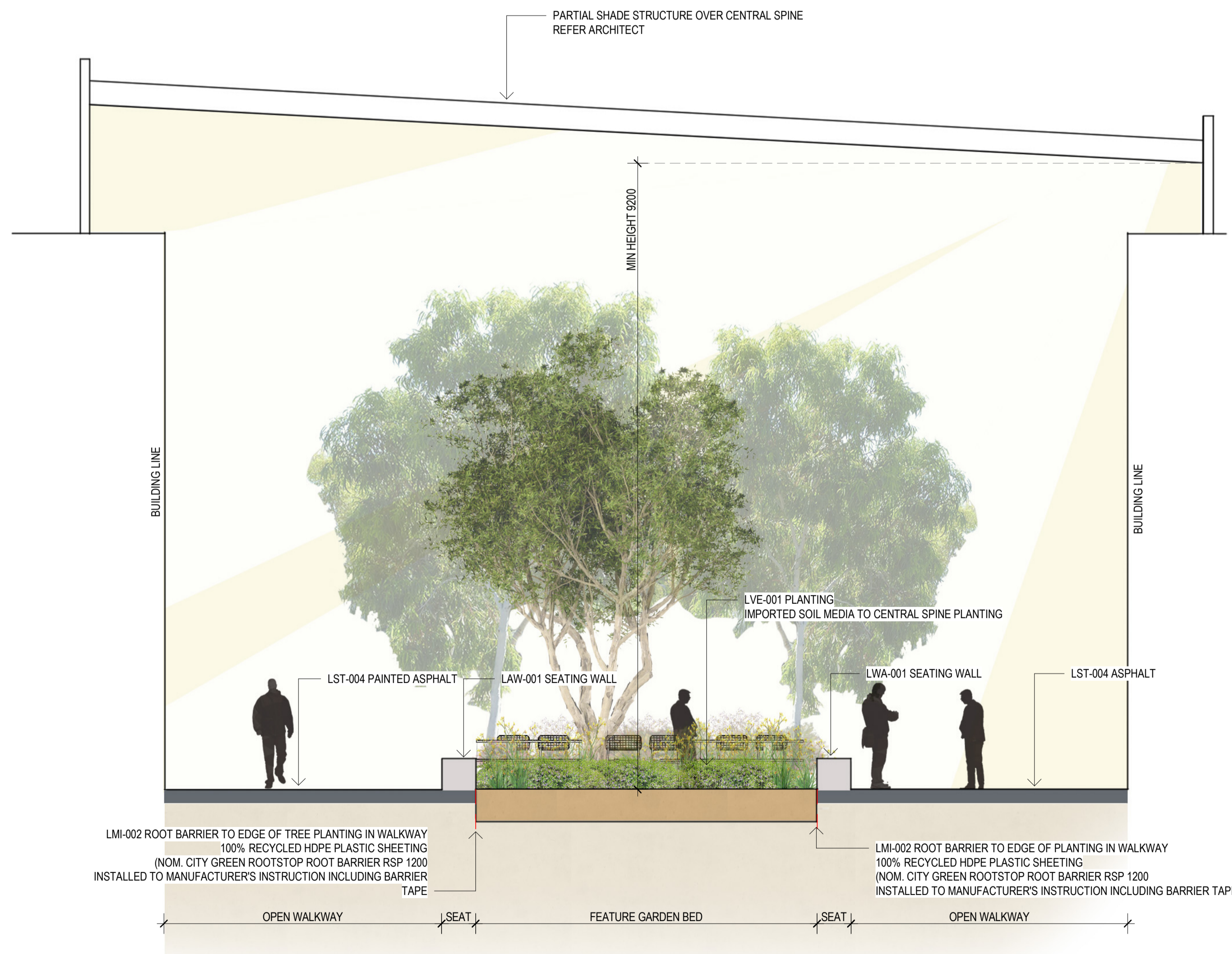
2 LANDSCAPE SPINE WALKWAY - TYPICAL CROSS SECTION 1:50
