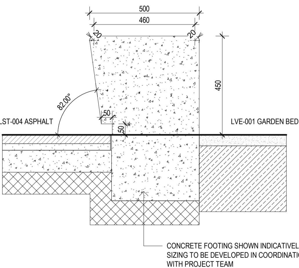
1 LWA-001 - INSITU CONCRETE SEATING WALL Copy 1 1:10
