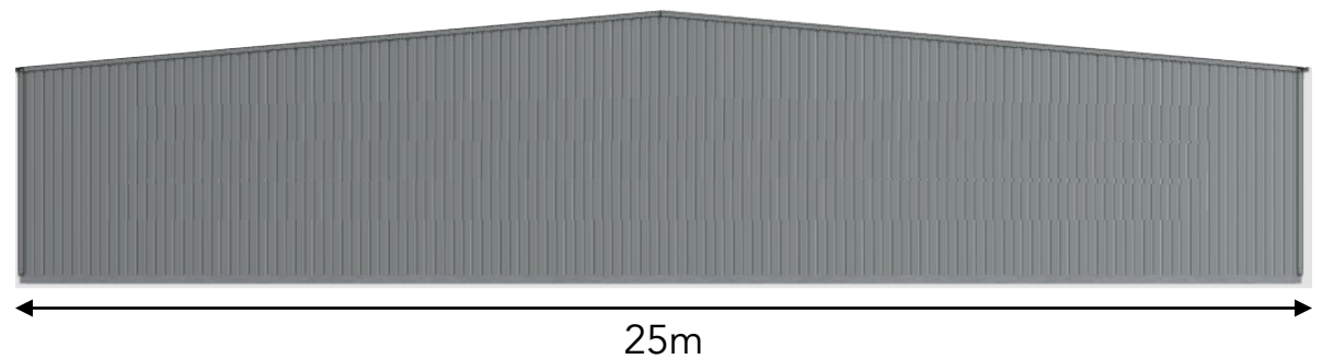
SOUTHERN ELEVATION
