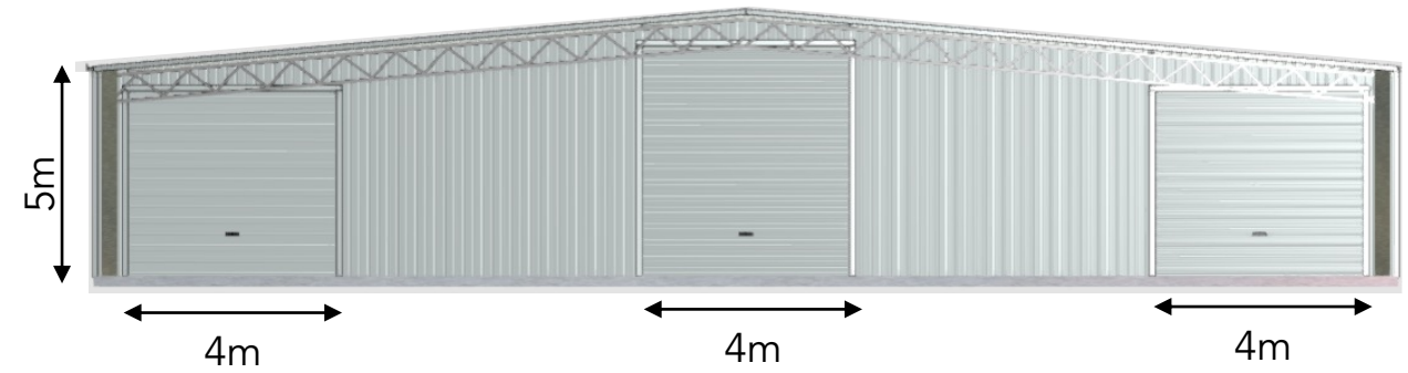
SOUTHERN ELEVATION
