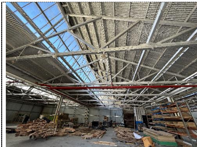
Figure 30. Saw tooth roof warehouse. The south facing saw tooth roof lights run the entire length of the bays in an east-west direction, facing south.
