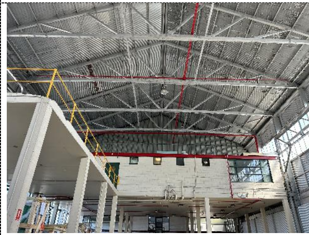
Figure 26. The 1989 mezzanine extends east of the brew house to accommodate offices, which have views out into the double height southern warehouse. The offices have metal cladding to the upper sections of the wall, steel trusses and concrete block walls below the windows.
