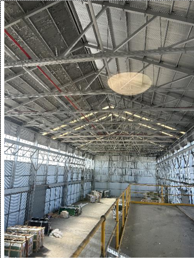
Figure 27. Southern warehouse, taken from the upper offices. The timber trusses have been painted silver.
